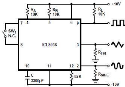
Fig. 8. High frequency oscillator circuit.
