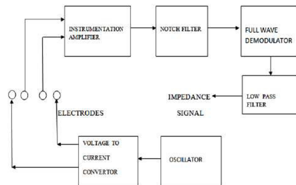
Fig. 7. Block diagram of impedance pneumography system.
