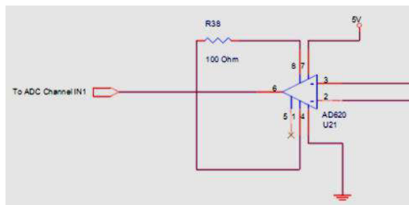
Fig. 3. Amplifier circuit using AD 620. Source: AD instruments 2018
